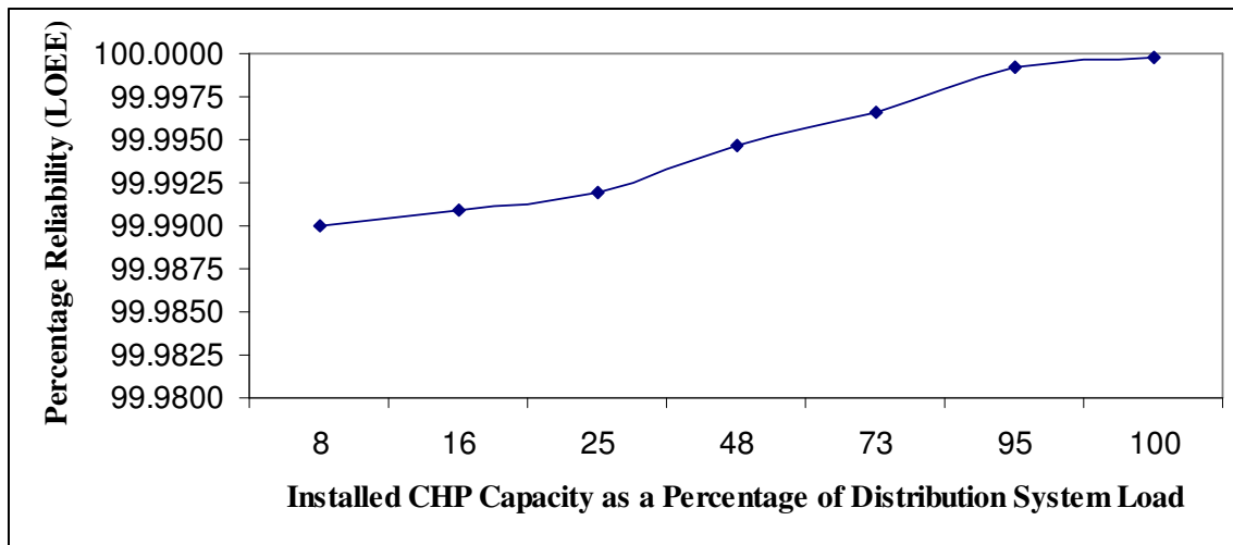
Figure 5.7: Percentage Reliability, LOEE - Case Study 3
